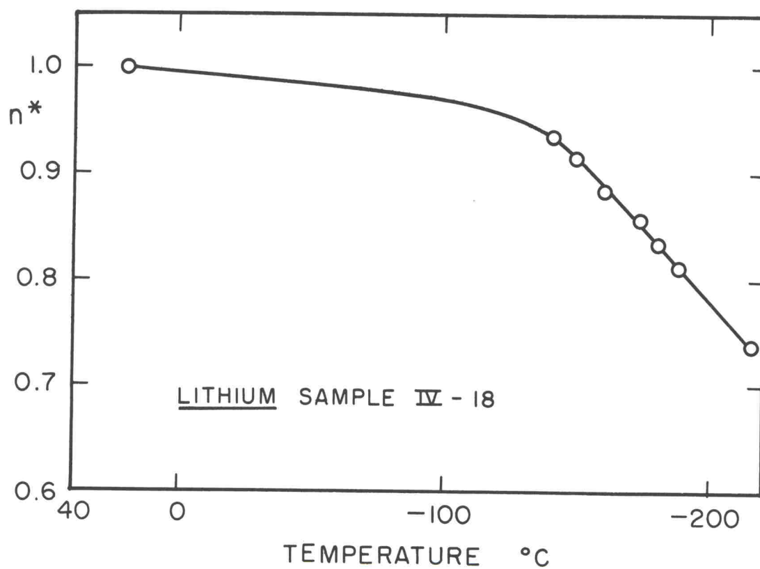
FIG. 3-15 n^* , NORMALIZED ELECTRONS/ATOM VS. TEMP.
